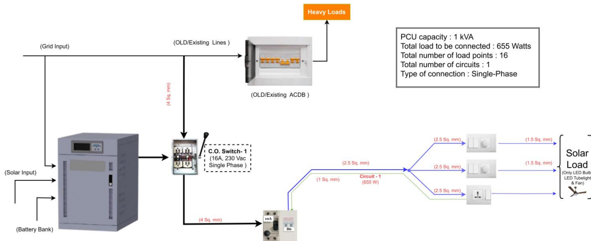
Load Wiring SLD For Sub Centre Option - 1
