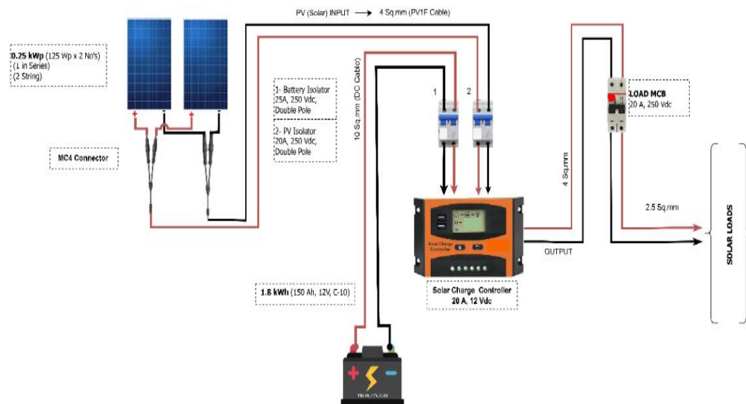
Solar System SLD For Sub Center/Staff Quaters
