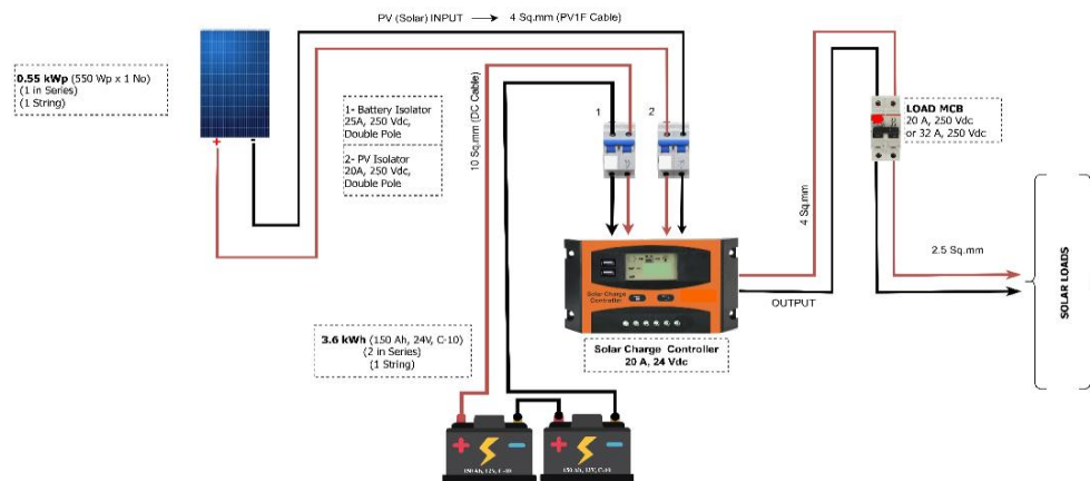
Solar System SLD For Sub Center Option 1
