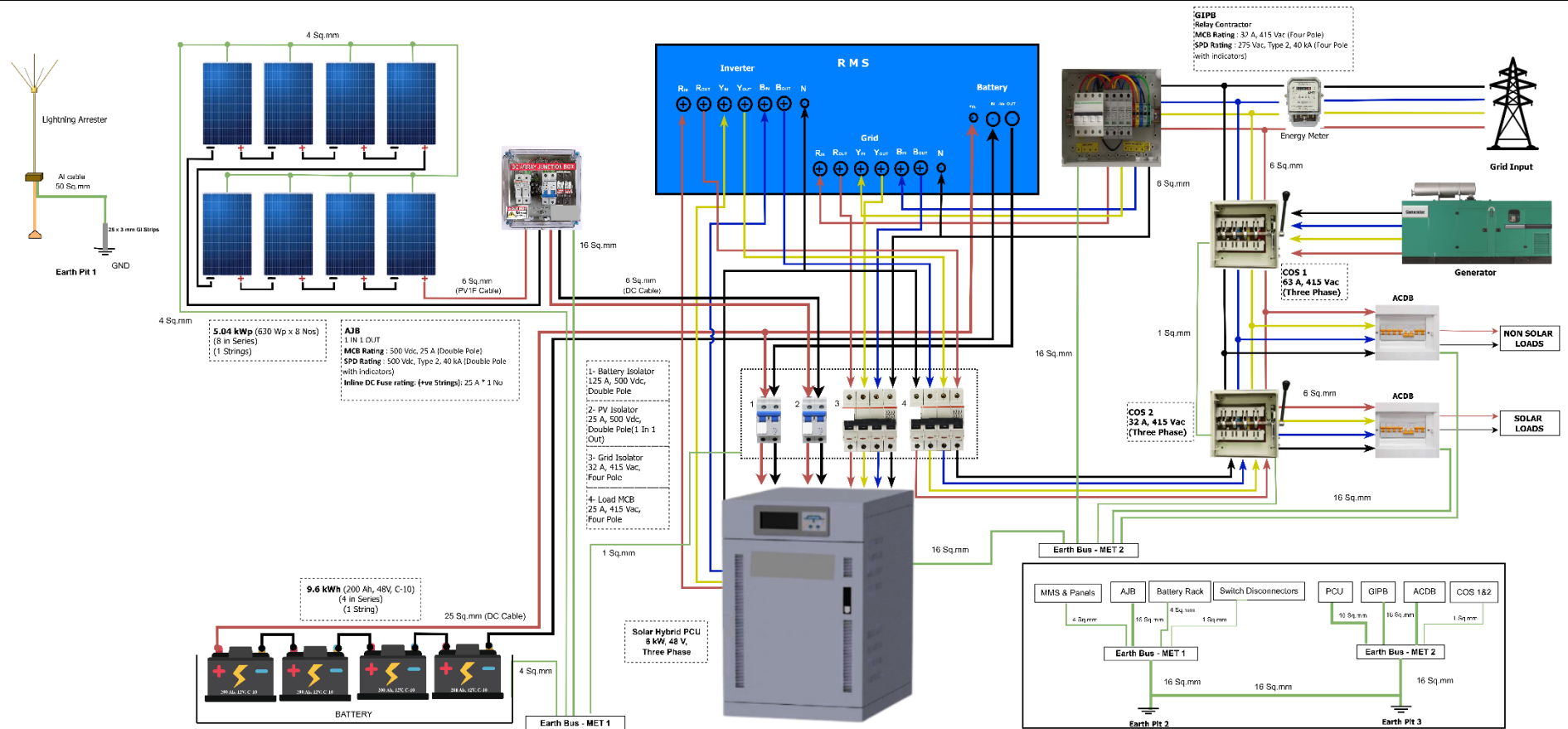
Solar System SLD For Primary Health Centre Option 2
