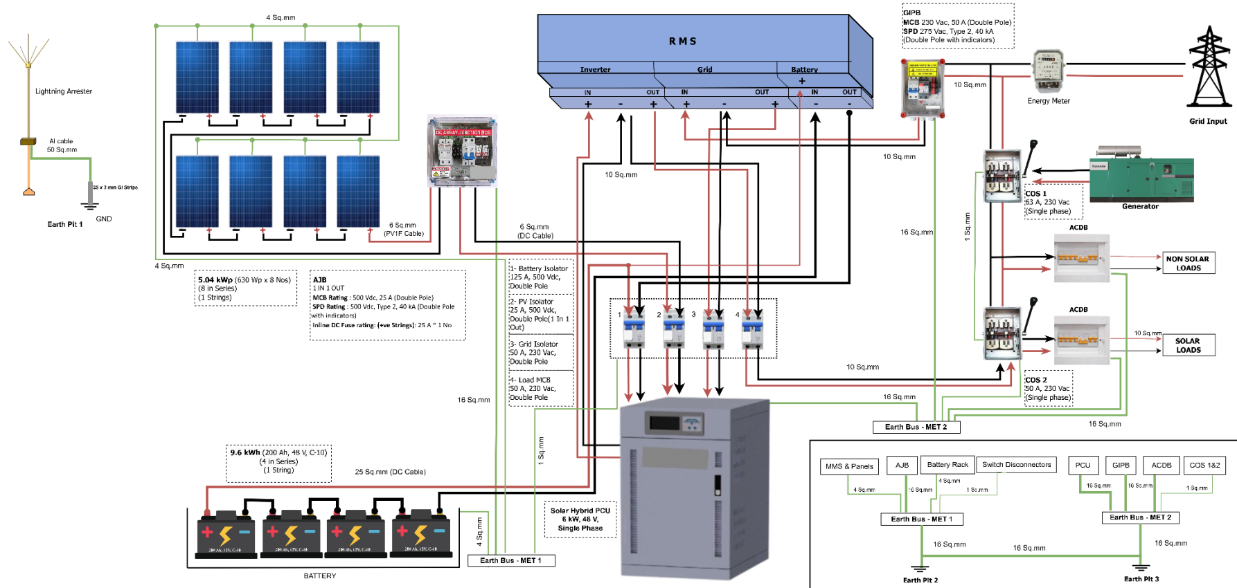
Solar System SLD For Primary Health Centre Option 1
